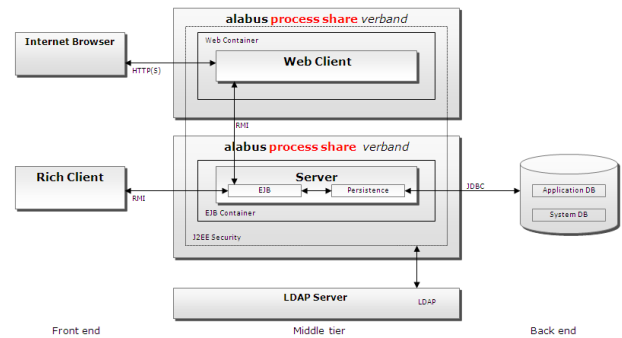
Architecture technique de la solution
